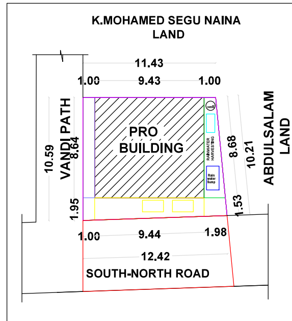
SITE PLAN & KEY PLAN (1:100)
