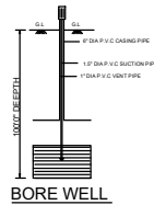
BORE WELL
