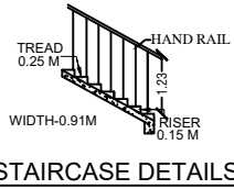
STAIRCASE DETAILS
