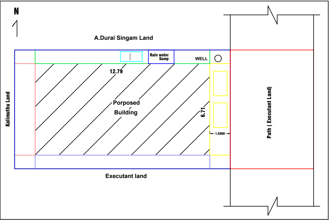
SITE PLAN CUM KEYPLAN
