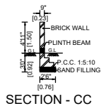
SECTION - CC
