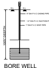
BORE WELL
