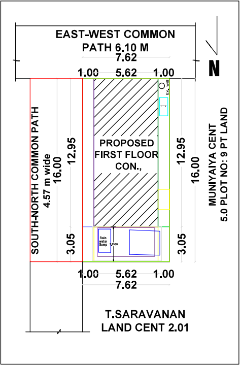
SITE PLAN & KEY PLAN (1:100)
