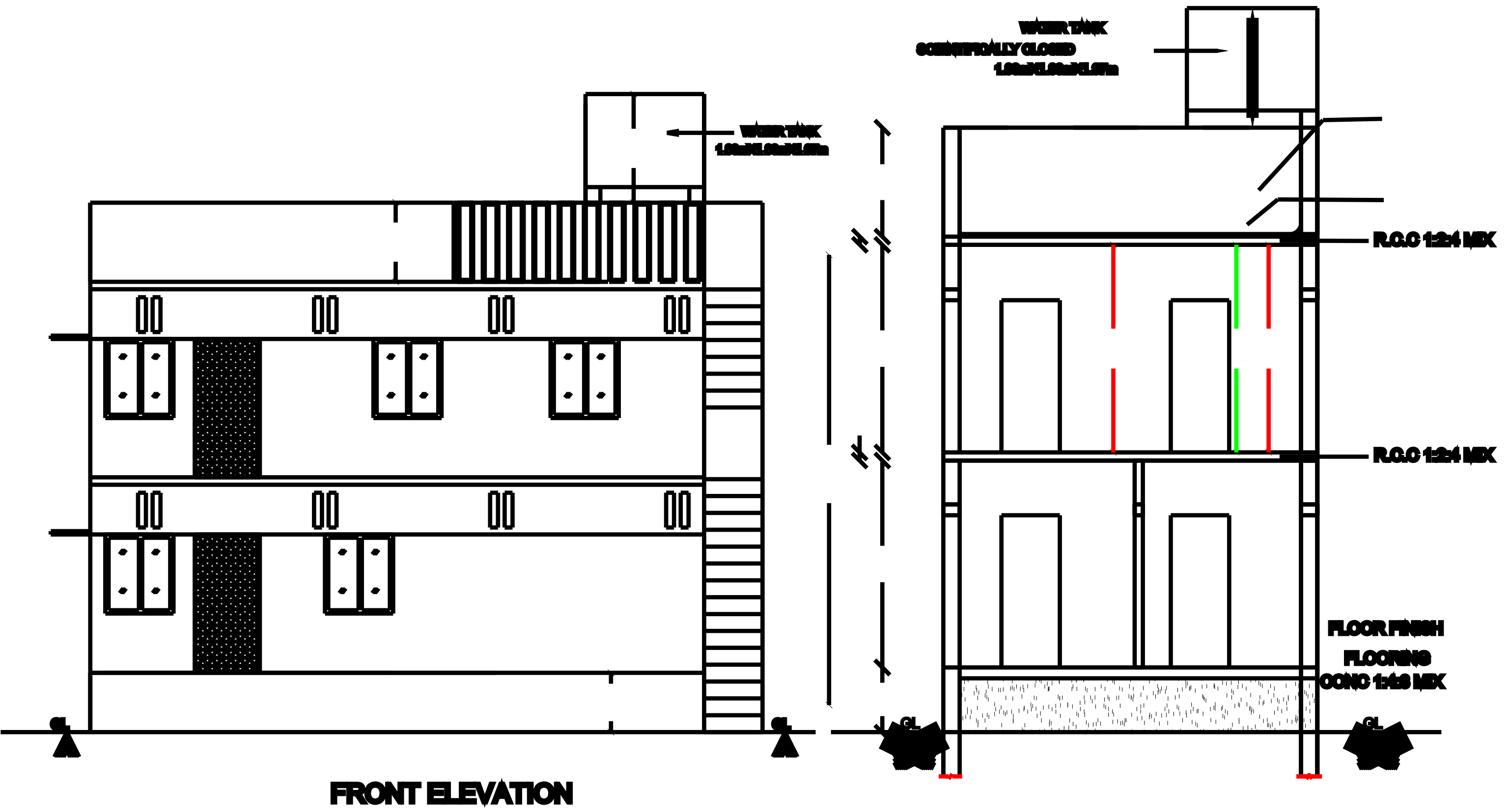
SECTION 'A-A'
