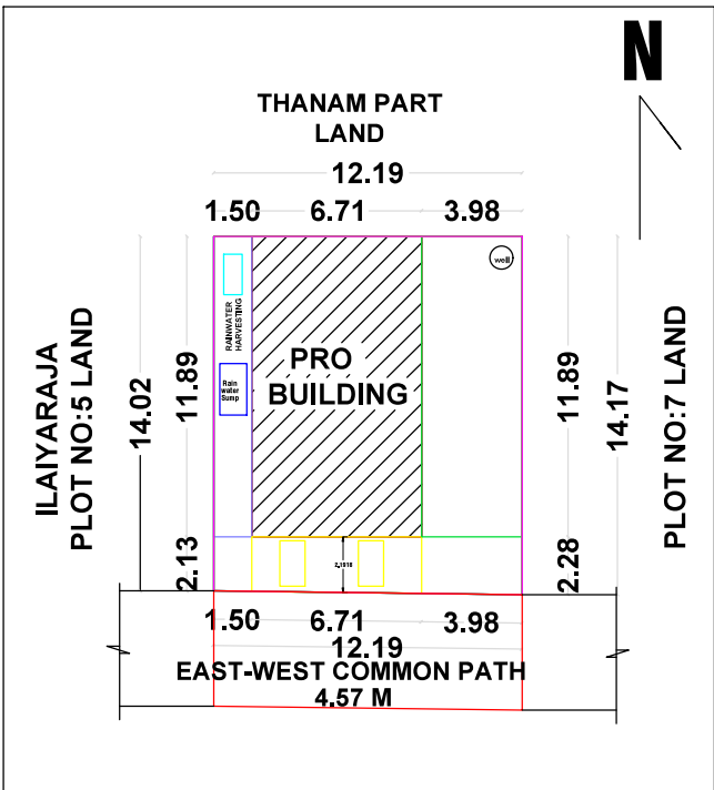
SITE PLAN & KEY PLAN (1:100)
