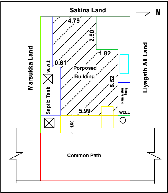
SITE PLAN CUM KEYPLAN
