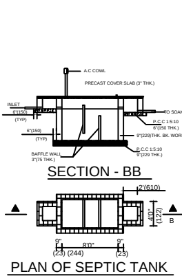
SECTION - BB PLAN OF SEPTIC TANK
