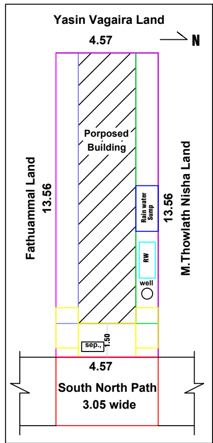
SITE PLAN CUM KEYPLAN
