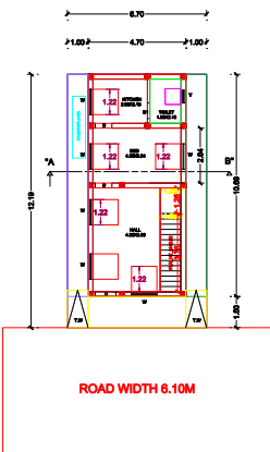
PRO. GROUND FLOOR PLAN
