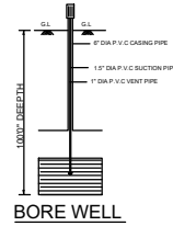
BORE WELL
