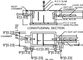
SEPTIC TANK:
