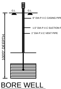
BORE WELL
