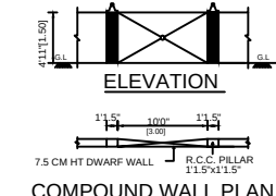
COMPOUND WALL PLAN
