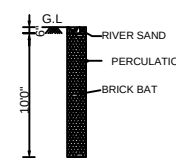
PERCOLATION PIT
