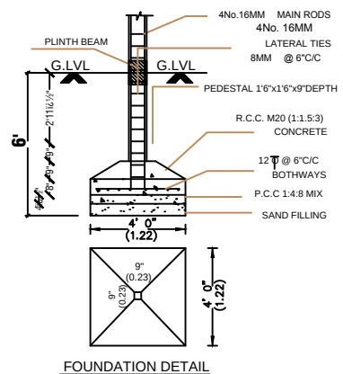
FOUNDATION DETAIL
