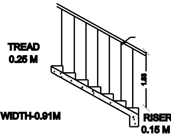
STAIRCASE DETAILS
