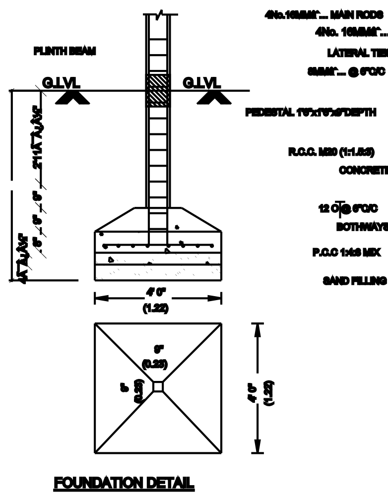
FOUNDATION DETAIL
