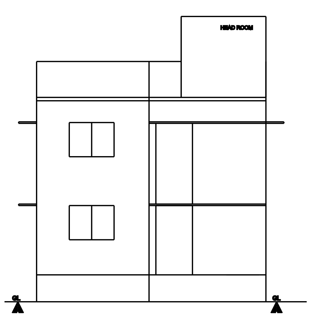
FRONT ELEVATION
