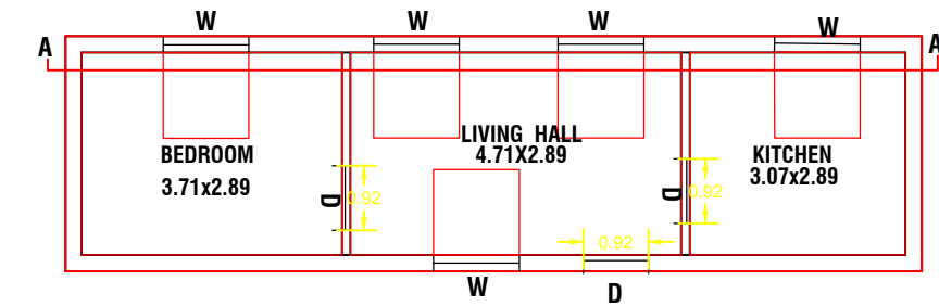
PRO., GROUND FLOOR PLAN
