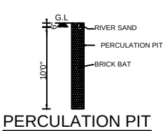
PERCOLATION PIT
