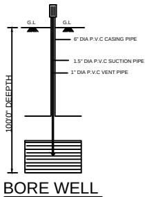
BORE WELL
