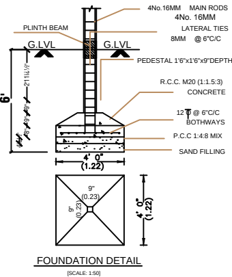
FOUNDATION DETAIL
