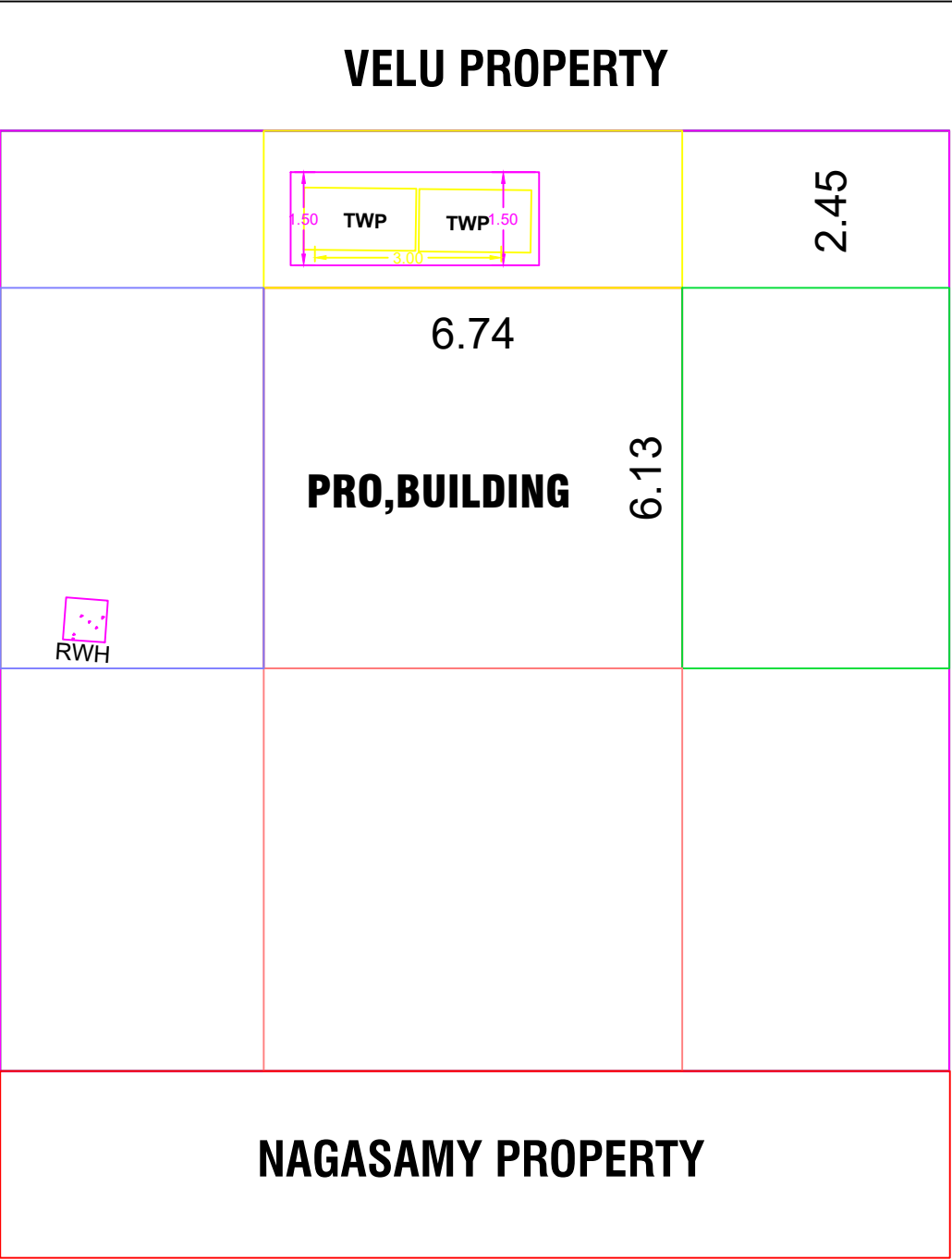
SITE PLAN
