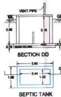
SEPTIC TANK
