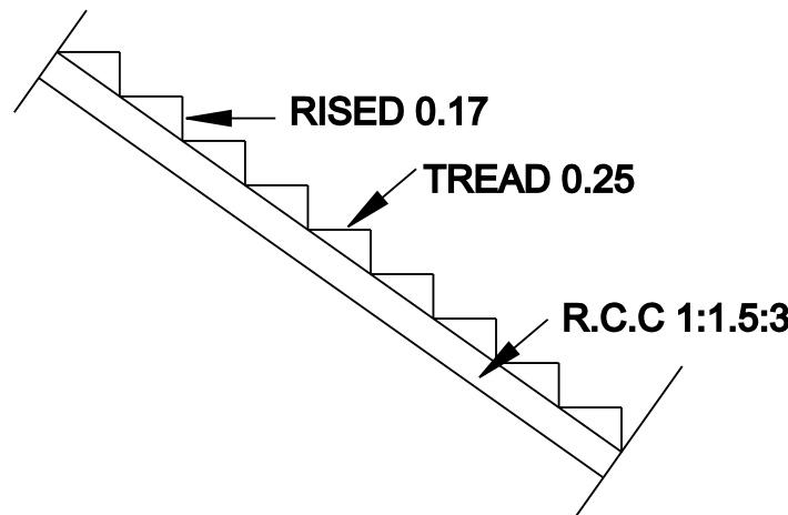
STAIRCASE DETAILS
