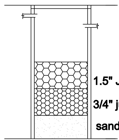
RAIN WATER HARVESTING TANK
