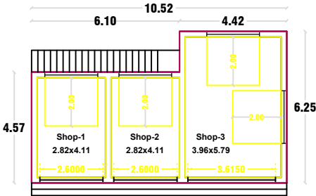
PRO. GROUND FLOOR PLAN
