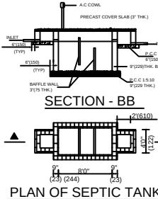
PLAN OF SEPTIC TANK
