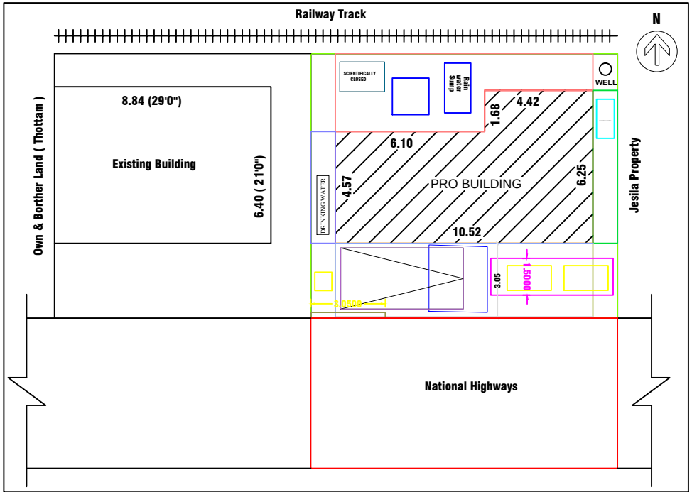
SITE PLAN & KEY PLAN
