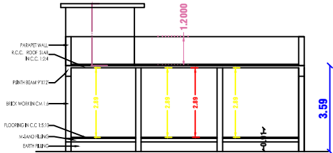
SECTION
