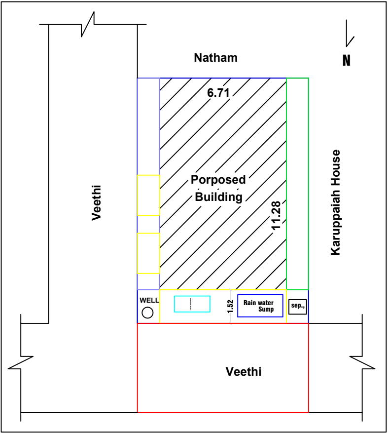
SITE PLAN CUM KEYPLAN
