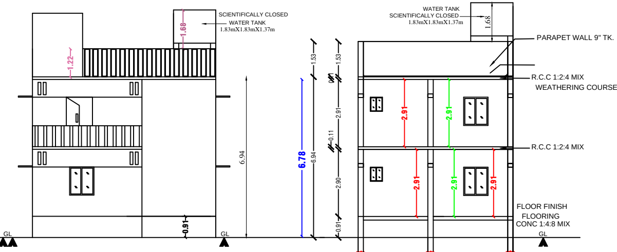
FRONT ELEVATION
