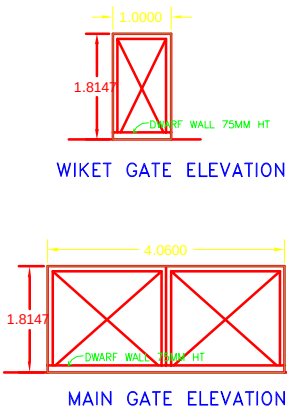
MAIN GATE ELEVATION
