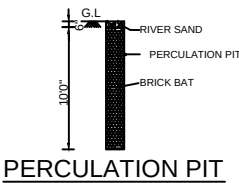
PERCOLATION PIT
