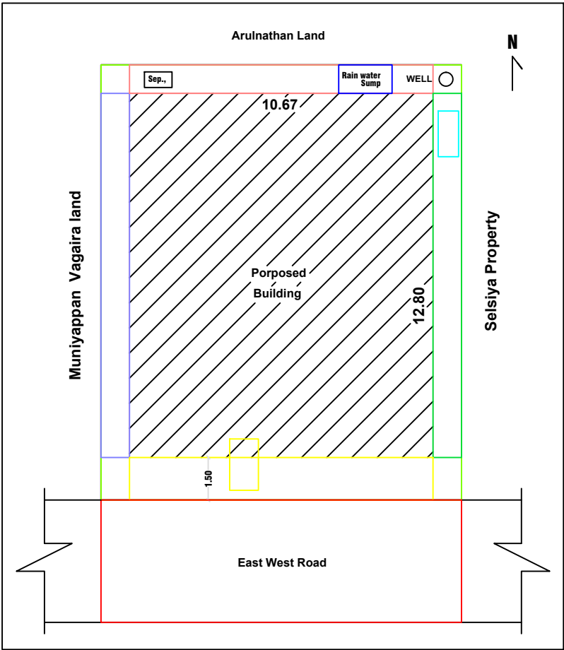
SITE PLAN CUM KEYPLAN
