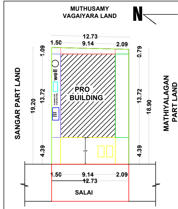
SITE PLAN & KEY PLAN (1:100)
