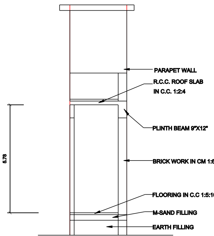
SECTION
