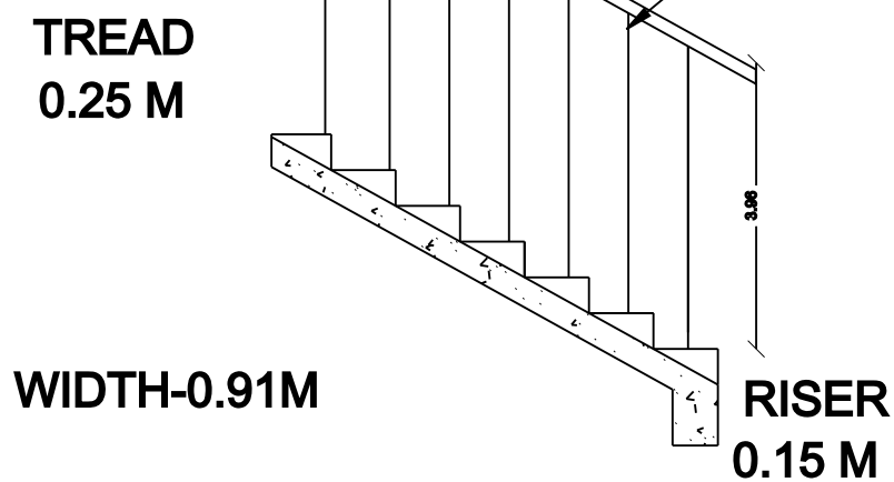
STAIRCASE DETAILS
