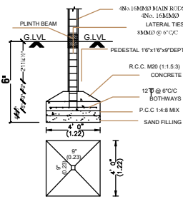
FOUNDATION DETAIL (SCALE: 1:50)
