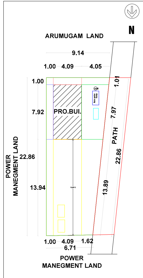
SITE PLAN & KEY PLAN
