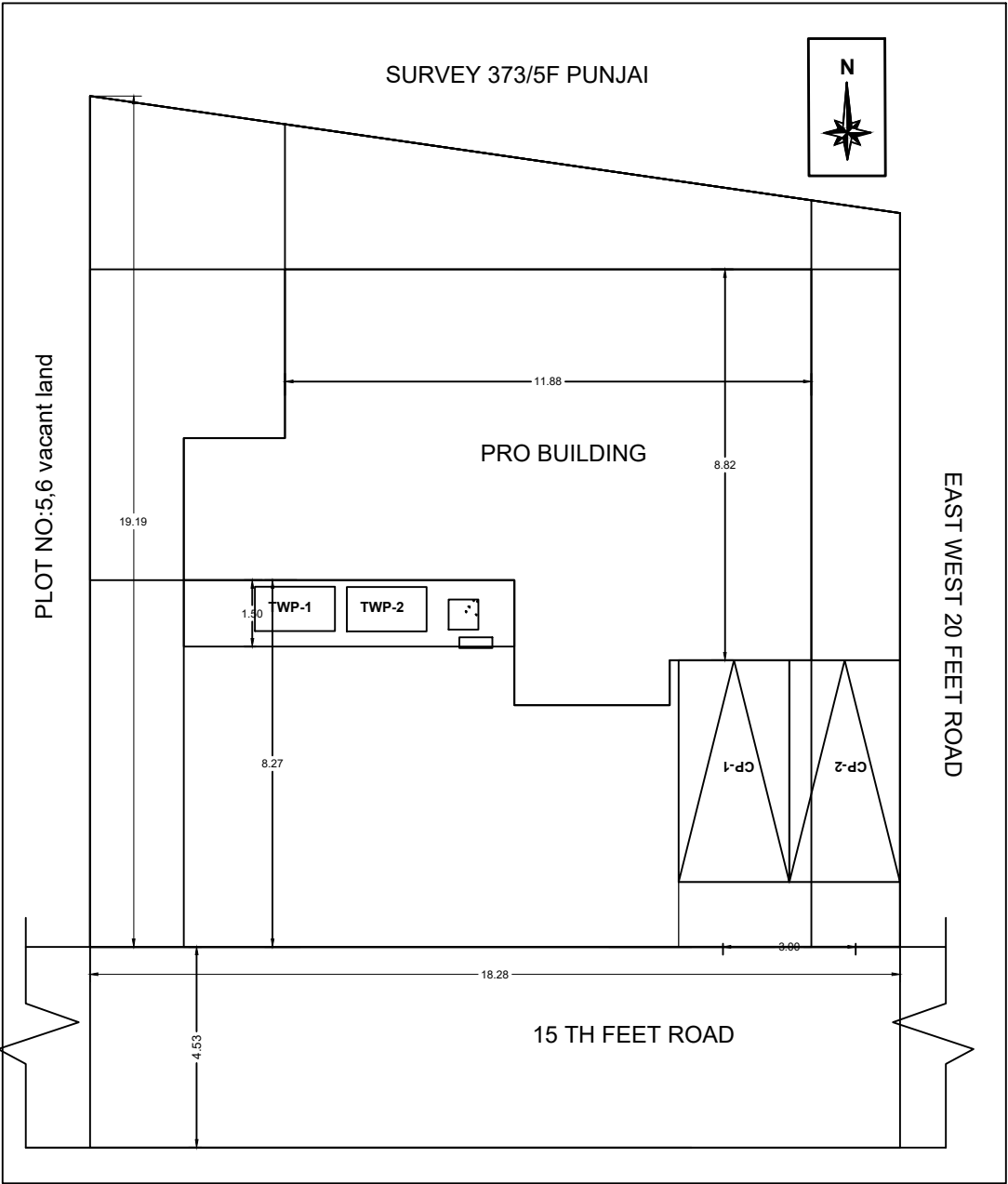
SITE PLAN
