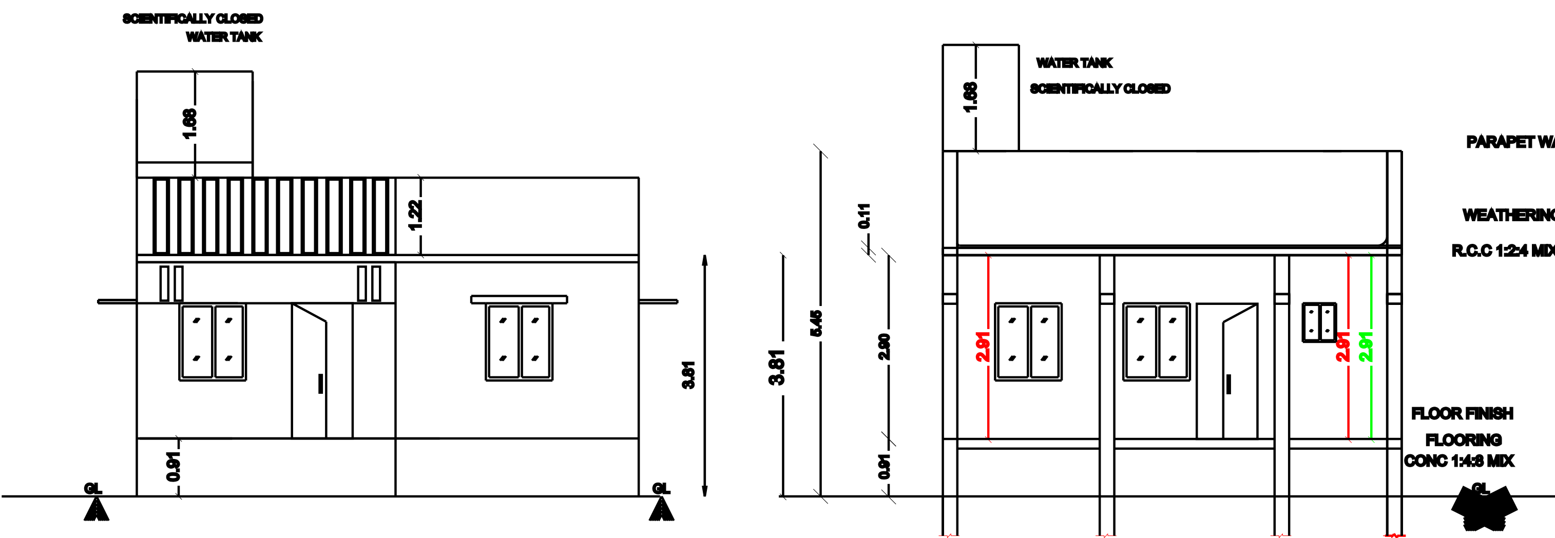
FRONT ELEVATION
