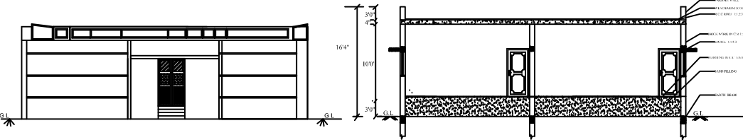
FRONT ELEVATION
