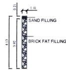
DETAILS OF PERCOLATION PIT
