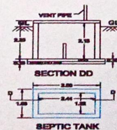
SEPTIC TANK
