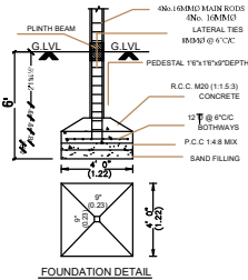
FOUNDATION DETAIL
