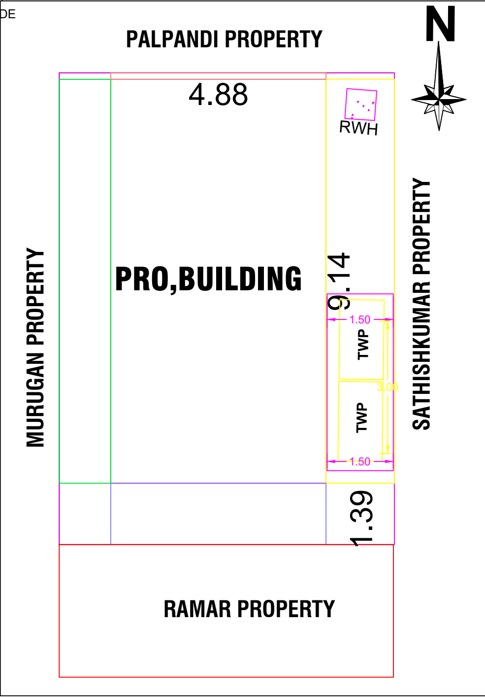
SITE PLAN
