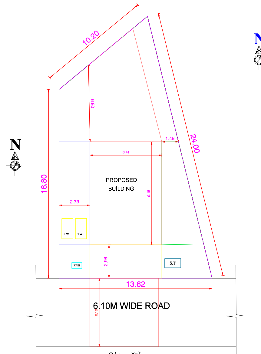
Site Plan
