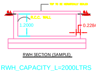
RWH_CAPACITY_L=2000LTRS
