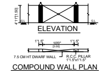
COMPOUND WALL PLAN
