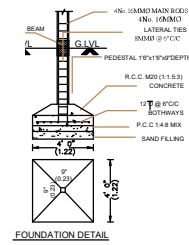
FOUNDATION DETAIL
