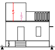
FRONT ELEVATION
