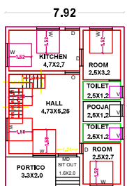
GROUND FLOOR PLAN
