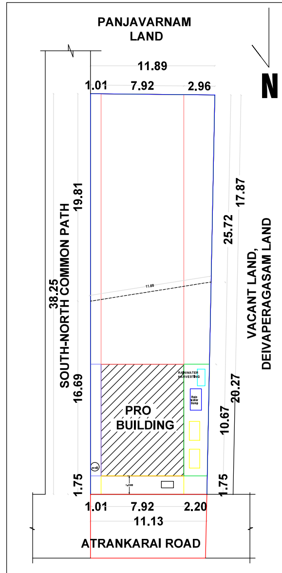
SITE PLAN & KEY PLAN (1:100)
