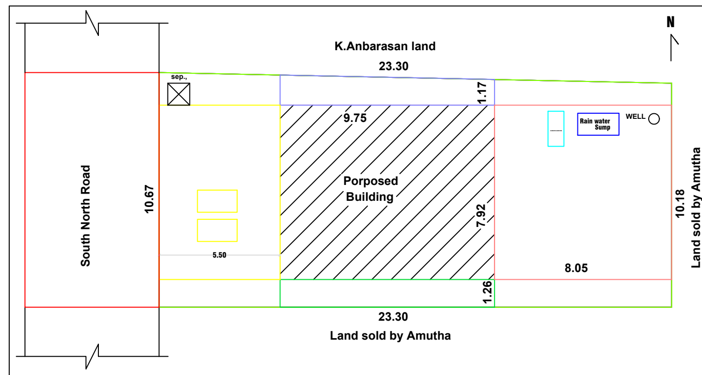
SITE PLAN CUM KEYPLAN
