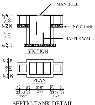
SEPTIC-TANK DETAIL
