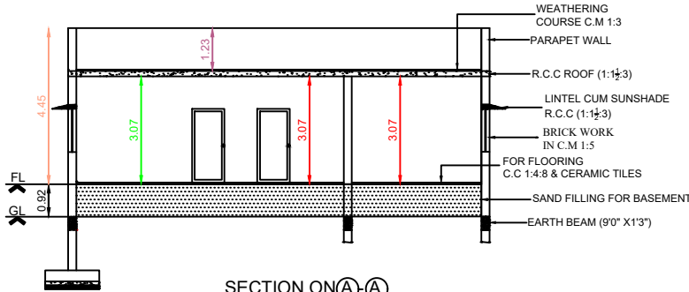
SECTION ON(A)-(A)
