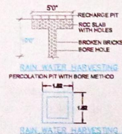
RAIN WATER HARVESTING PLAN
