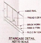
STAIRCASE DETAIL NOT TO SCALE
