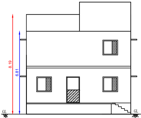
FRONT ELEVATION
