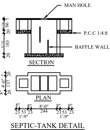
SEPTIC-TANK DETAIL
