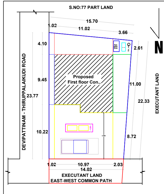
SITE PLAN & KEY PLAN (1:100)
