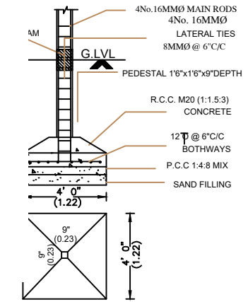
FOUNDATION DETAIL (SCALE: 1:50)
