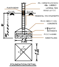
FOUNDATION DETAIL
