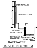
RAIN WATER HARVESTING SYSTEM
