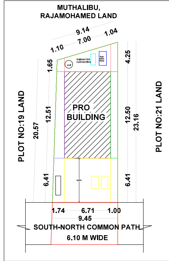
SITE PLAN & KEY PLAN (1:100)
