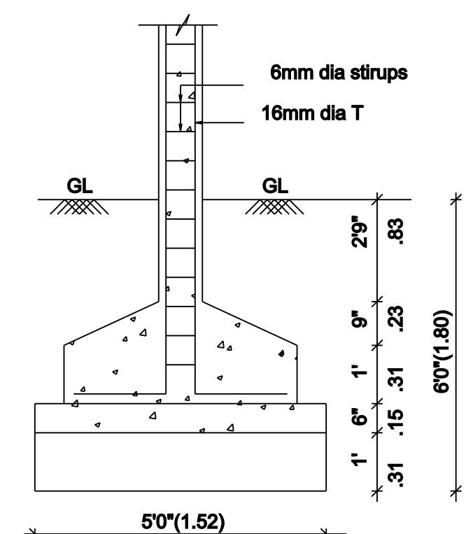
COLUMN FOUNDATION DETAIL
