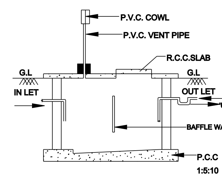
SEC. OF SEPTIC TANK
