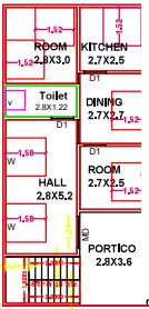
GROUND FLOOR PLAN
