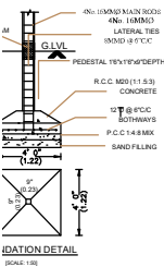
FOUNDATION DETAIL
