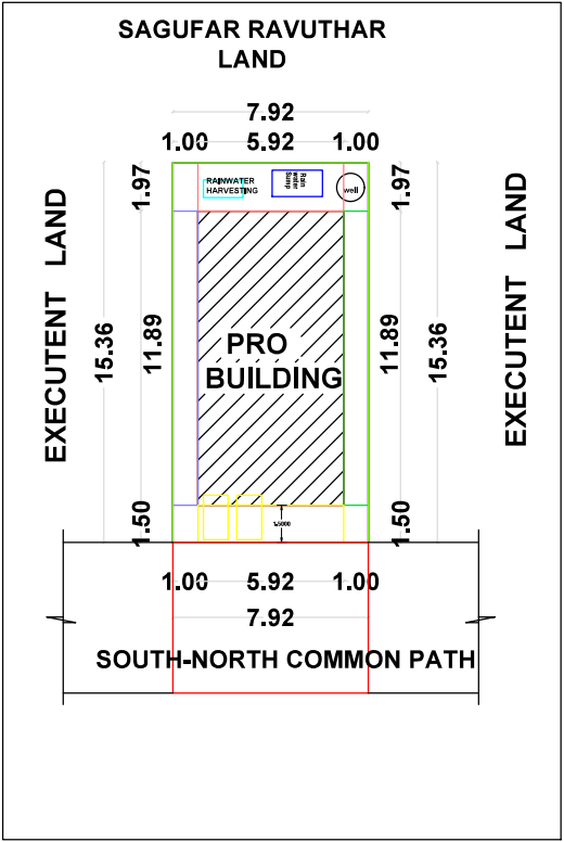
SITE PLAN & KEY PLAN (1:100)
