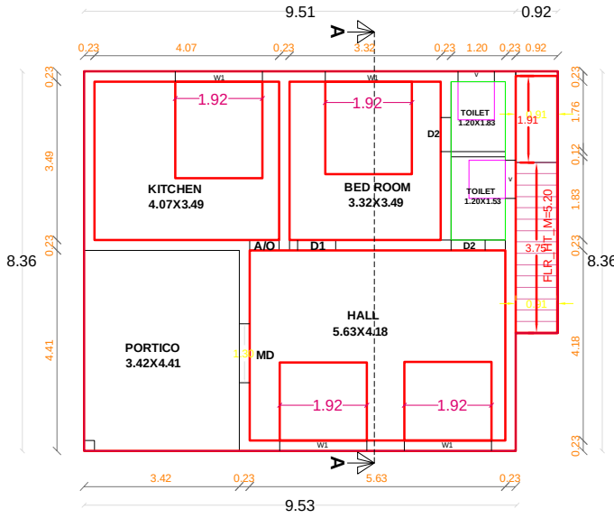
GROUND FLOOR PLAN PROPOSED
