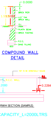
COMPOUND WALL DETAIL
