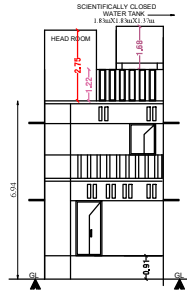
FRONT ELEVATION
