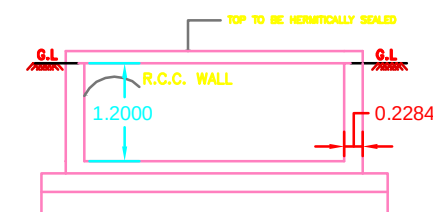
RWH SECTION (SAMPLE)
