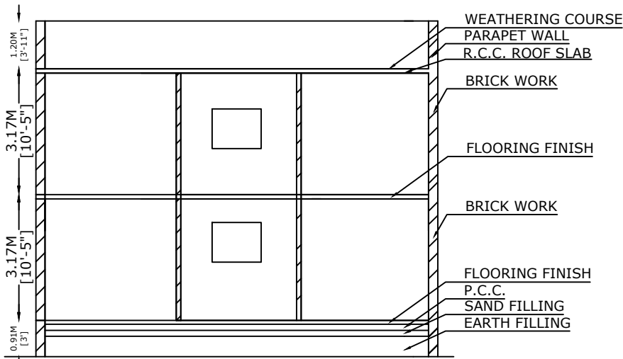
SECTION AN AA
