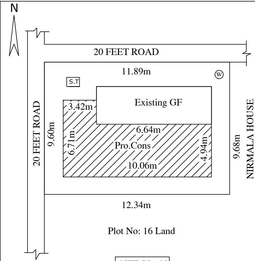
SITE PLAN
