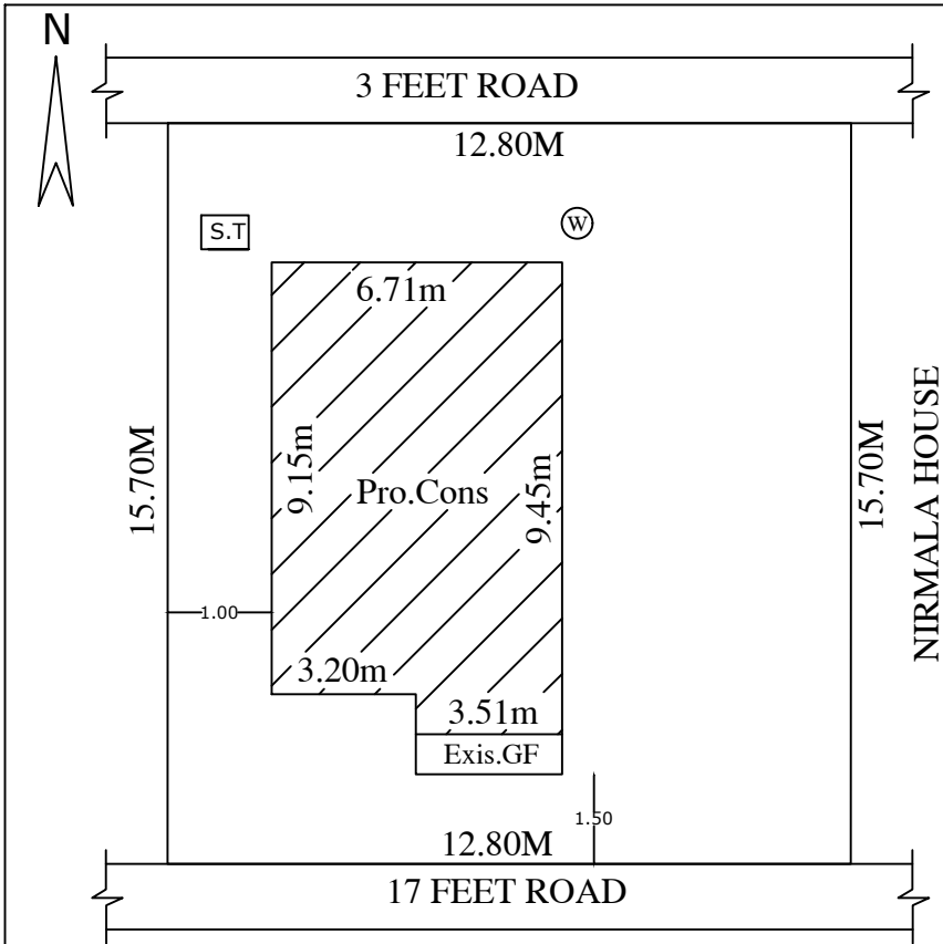
SITE PLAN
