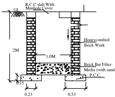
Collection Pit (Recharge Well Method) SCALE:- 1"=4'0"
