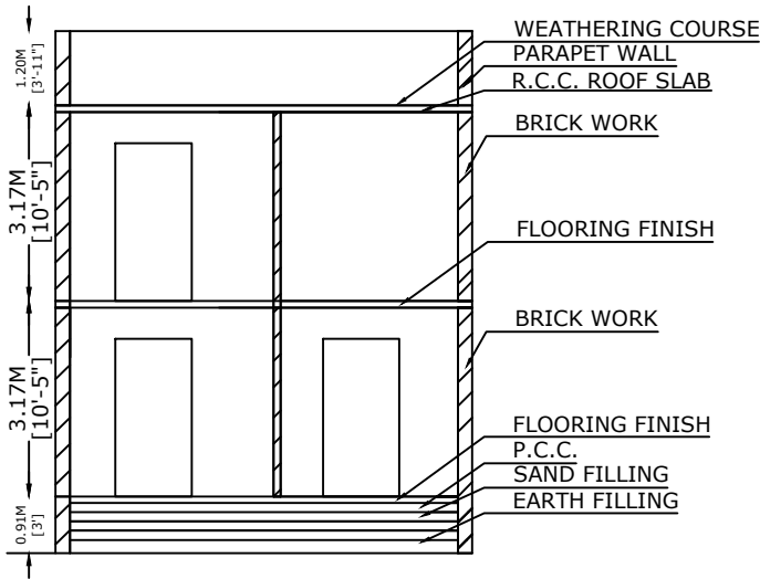
SECTION AN AA
