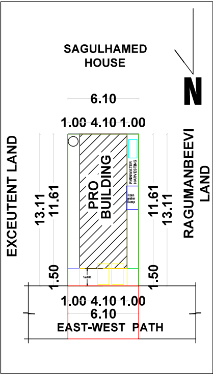
SITE PLAN & KEY PLAN (1:100)
